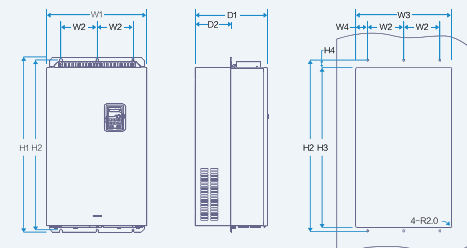
3-phase 220VAC series 75-110kW Flange mounting Installation diagram
