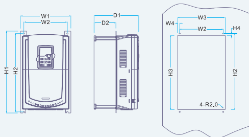
3-phase 220VAC series 11-15kW Flange mounting Installation diagram
