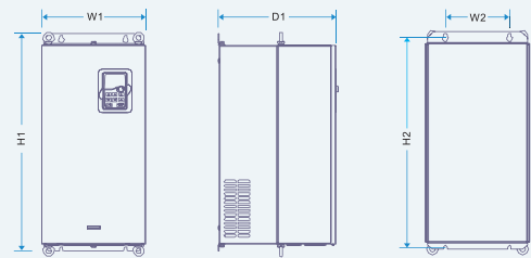
3-phase 220VAC series 18.5-55kW Flange mounting Installation diagram
