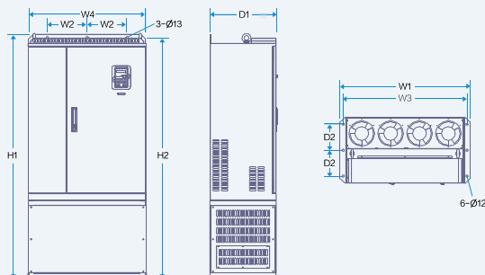
3-phase 220VAC series 132-160kW Floor mounting Installation diagram
