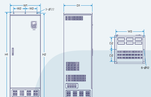
3-phase 220VAC series 185-250kW Floor mounting Installation diagram
