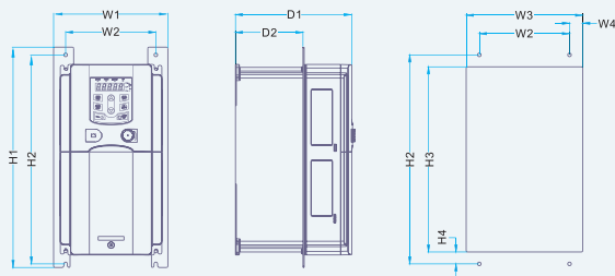
3-phase 220VAC series 0.75-7.5kW Flange mounting Installation diagram
